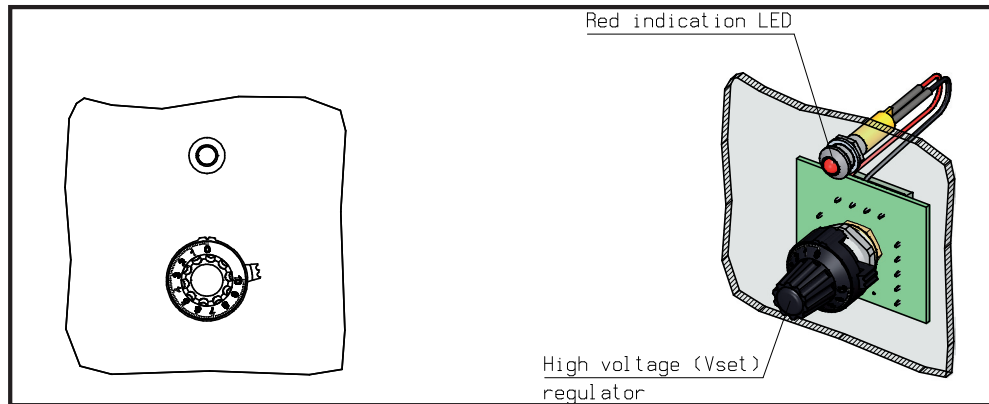
Technische tekening External control kit Perfomaster
